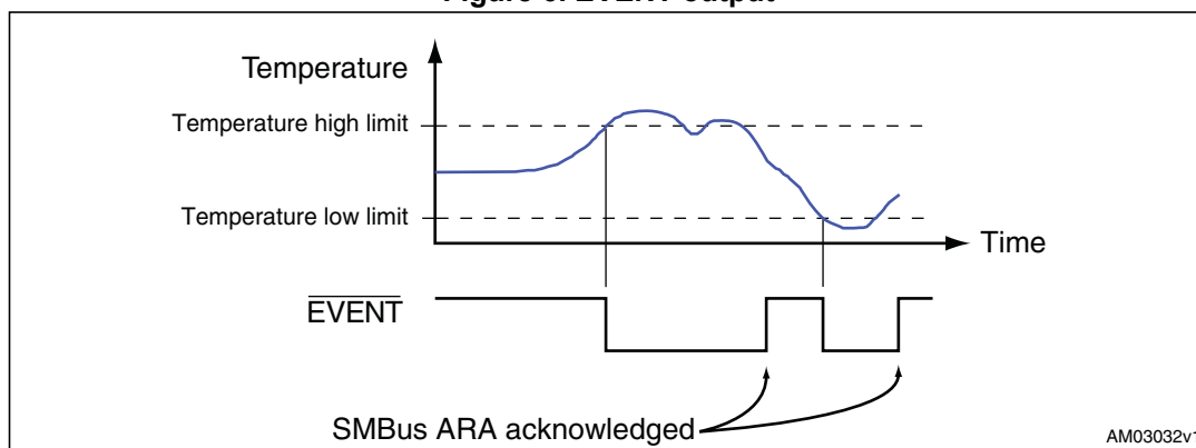
Figure 6. \overline{\text{EVENT}} output
