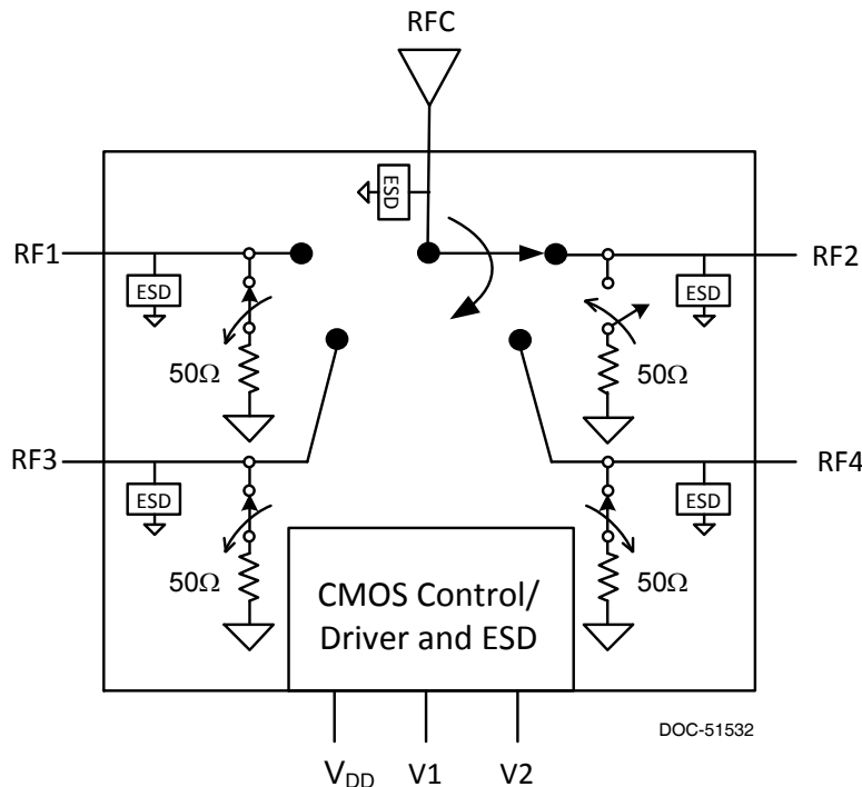
Figure 1. Functional Diagram
