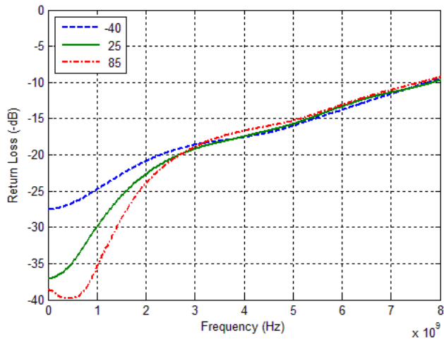
Figure 12. Terminated Port Return Loss vs. Temp
