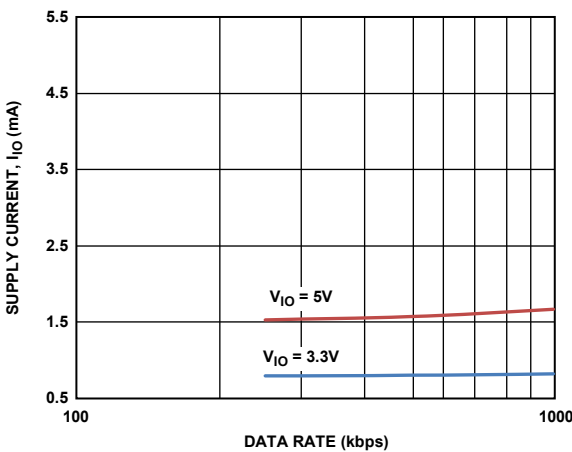
Figure 7. Supply Current, I_{IO} vs. Data Rate
