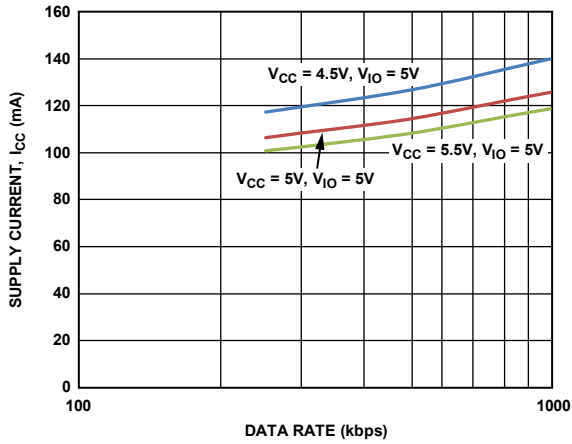
Figure 5. Supply Current, I_{CC} vs. Data Rate
