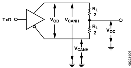
Figure 22. Driver Voltage Measurement
