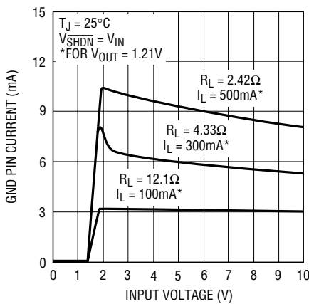
LT1764A GND Pin Current
