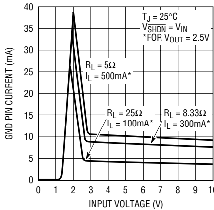
LT1764A-2.5 GND Pin Current
