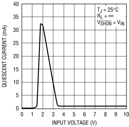
LT1764A-3.3 Quiescent Current
