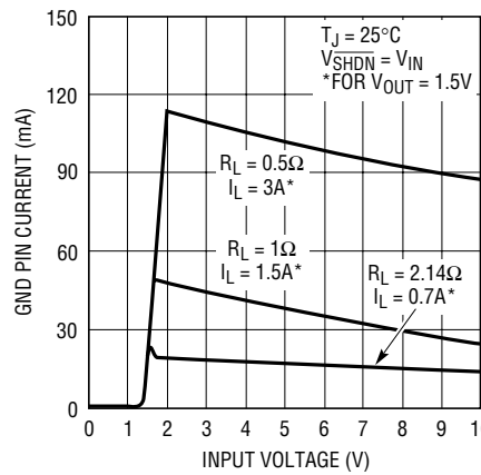
LT1764A-1.5 GND Pin Current
