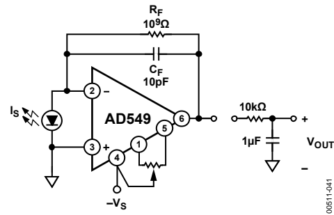
Figure 41. Photodiode Preamp
