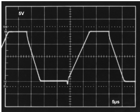
Figure 20. Unity-Gain Follower Large Signal Pulse Response
