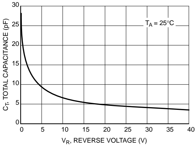
Figure 4. Total Capacitance
