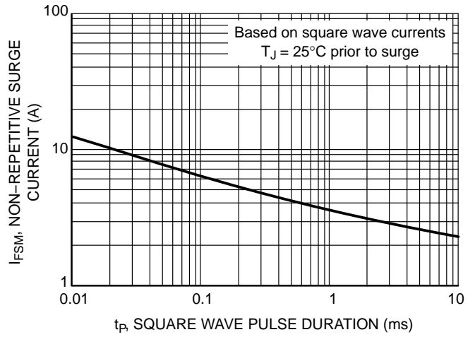
Figure 5. Non-Replicative Surge Current
