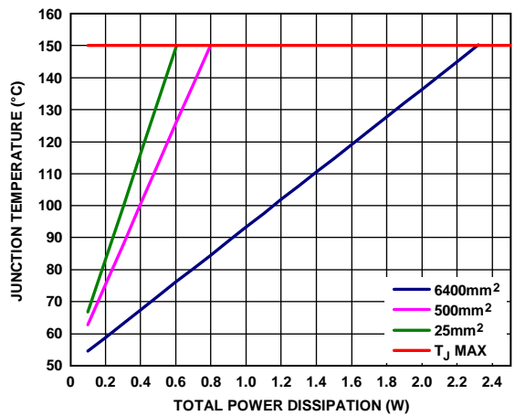
Figure 66. LFCSP, TA = 50°C
