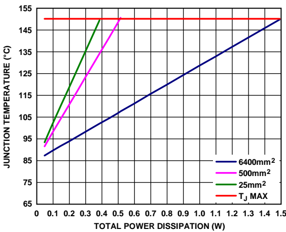
Figure 67. LFCSP, TA = 85°C
