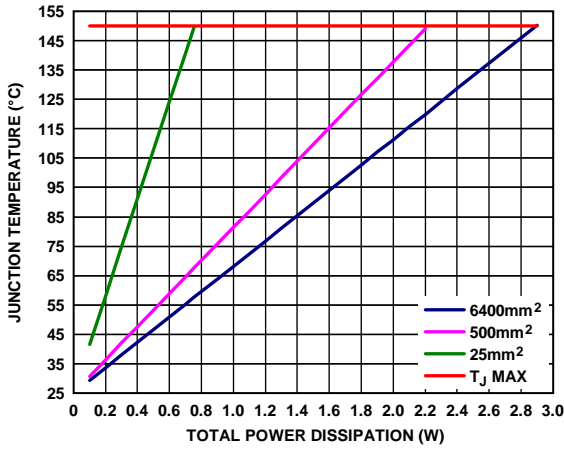
Figure 65. LFCSP, TA = 25°C
