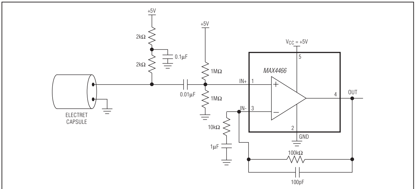
Figure 2. MAX4466 Typical Application Circuit
