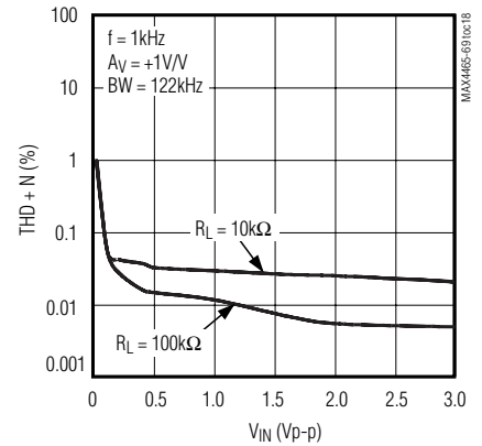
MAX4465/MAX4467/MAX4469 TOTAL HARMONIC DISTORTION PLUS NOISE vs. INPUT AMPLITUDE
