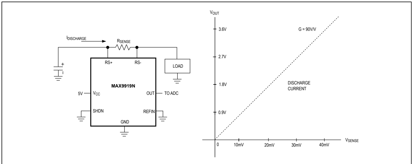
Figure 1. Unidirectional Operation
