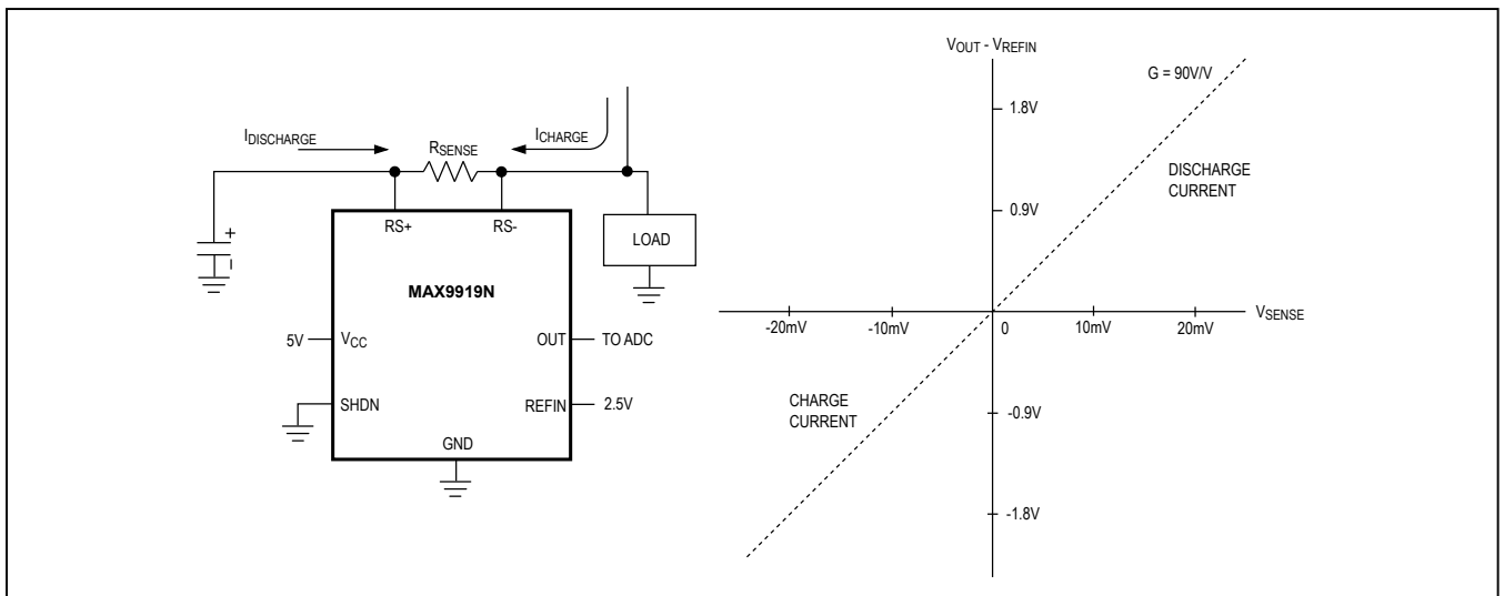
Figure 2. Bidirectional Operation
