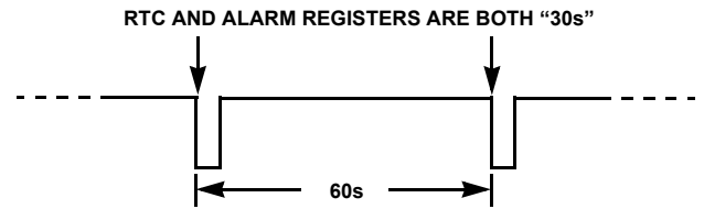
FIGURE 15. \overline{IRQ}/F_{OUT} WAVEFORM
