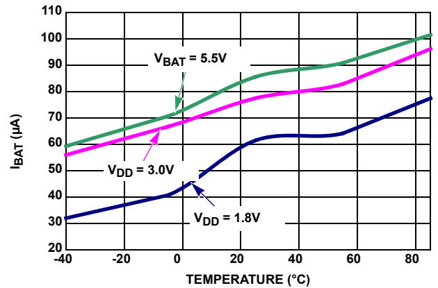
FIGURE 10. I BAT WITH TSE = 1, BTSE = 1 vs TEMPERATURE
