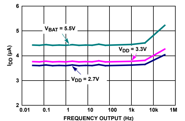
FIGURE 8. F_{OUT} vs I_{DD}
