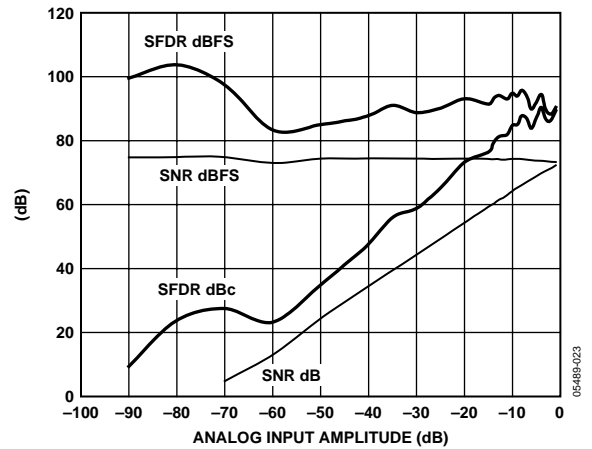
Figure 23. AD9445-125 SNR/SFDR vs. Analog Input Level, 125 MSPS/225.3 MHz, CMOS Output Mode
