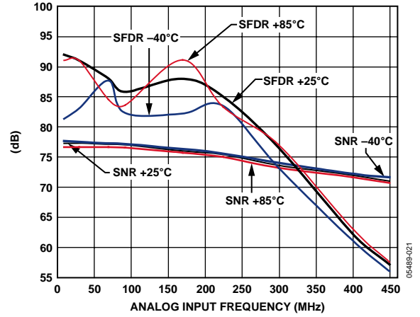
Figure 21. AD9445-125 SNR/SFDR vs. Analog Input Frequency, 125 MSPS, 3.2 V p-p Input Range
