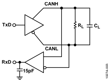
Figure 23. Switching Characteristics Measurements
