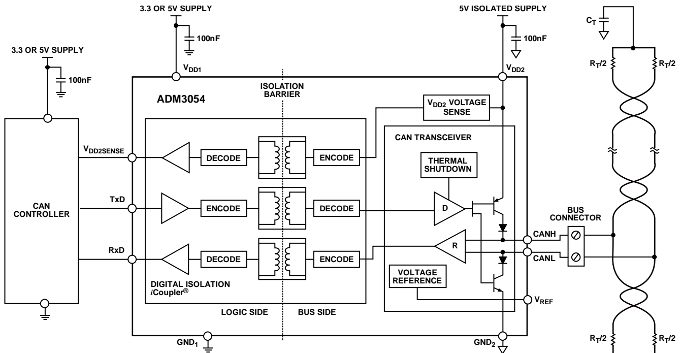
Figure 32. Typical Isolated CAN Node Using the ADM3054
