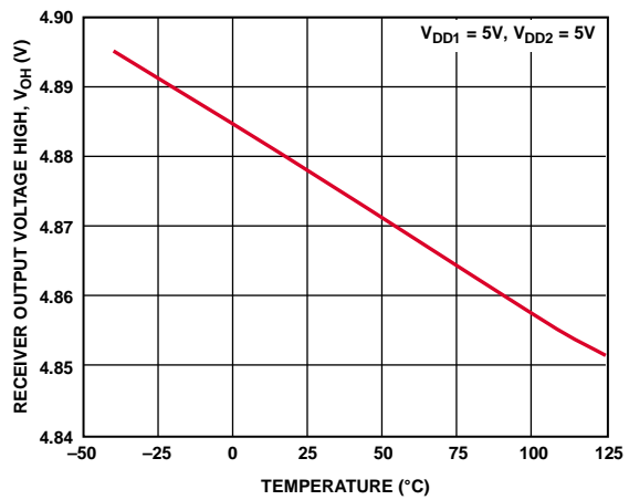
Figure 16. Receiver Output High Voltage vs. Temperature
