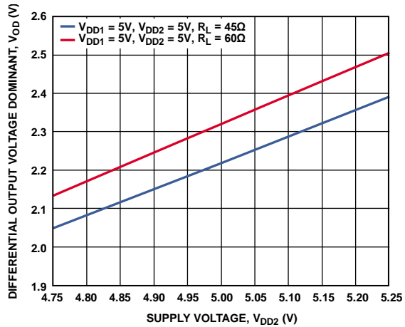
Figure 15. Driver Differential Output Voltage Dominant vs. Supply Voltage, V_{DD2}
