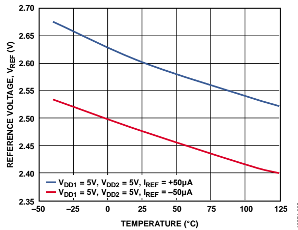
Figure 18. V_{REF} vs. Temperature
