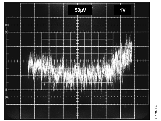
Figure 65. Gain Nonlinearity vs. Output Voltage, G = -10 , RM-8 and R-8 Package Options
