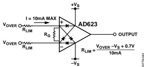
Figure 73. Input Protection
