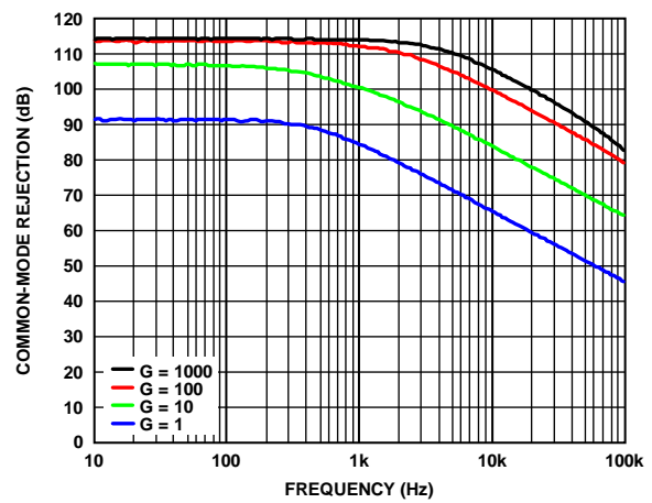
Figure 25. Common-Mode Rejection vs. Frequency, +V_S = 5\text{ V} , -V_S = 0\text{ V} , V_{REF} = 2.5\text{ V} , for Various Gain Settings, RM-8 and R-8 Package Options
