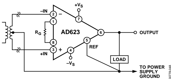
Figure 78. Ground Returns for Bias Currents with Transformer-Coupled Inputs
