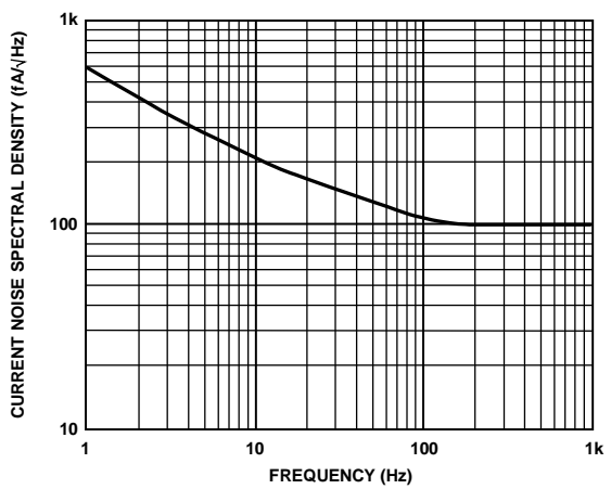
Figure 16. Current Noise Spectral Density vs. Frequency, N-8 Package Option
