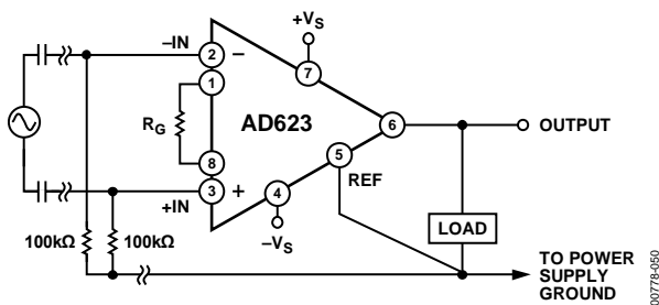
Figure 80. Ground Returns for Bias Currents with AC-Coupled Inputs
