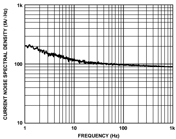
Figure 17. Current Noise Spectral Density vs. Frequency, RM-8 and R-8 Package Options
