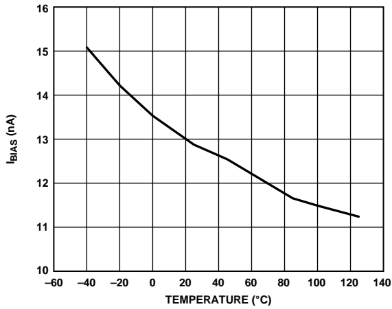
Figure 15. I_{BIAS} vs. Temperature, RM-8 and R-8 Package Options
