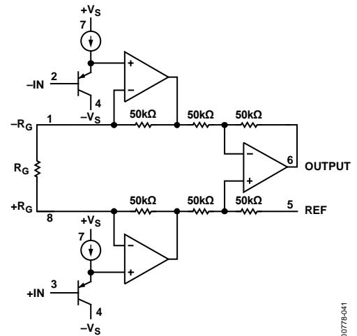
Figure 70. Simplified Schematic
