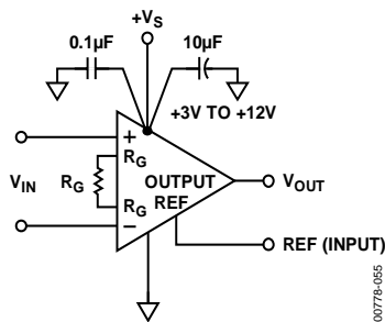
Figure 72. Single-Supply Basic Connection
