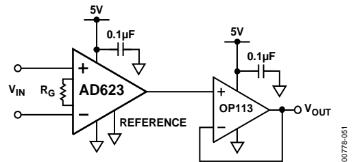
Figure 81. Output Buffering
