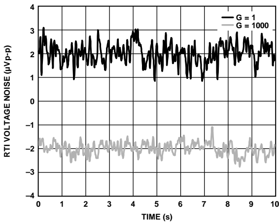
Figure 23. RTI Voltage Noise, 0.1 Hz to 10 Hz vs. Time, RM-8 and R-8 Package Options
