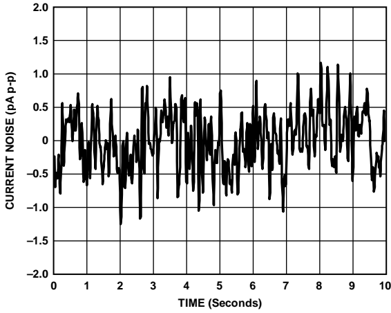
Figure 21. 0.1 Hz to 10 Hz Current Noise vs. Time, RM-8 and R-8 Package Option
