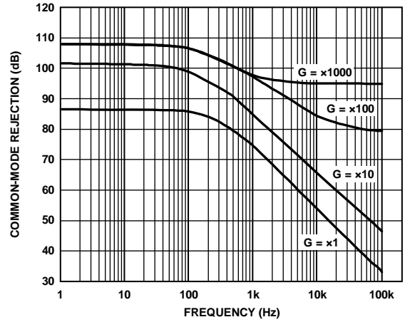
Figure 24. Common-Mode Rejection vs. Frequency, +V_S = 5\text{ V} , -V_S = 0\text{ V} , V_{REF} = 2.5\text{ V} , for Various Gain Settings, N-8 Package Option
