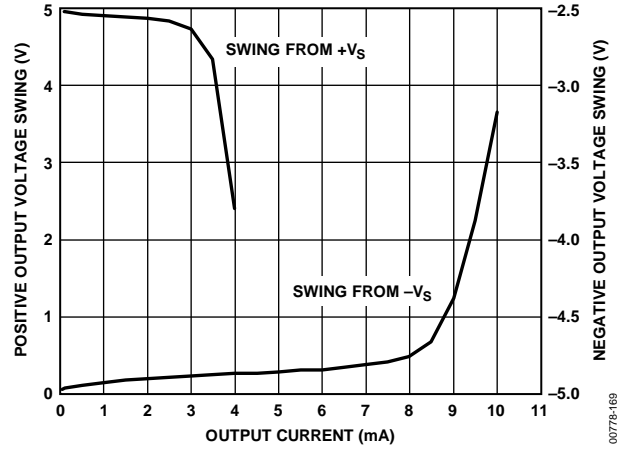
Figure 69. Positive and Negative Output Voltage Swing vs. Output Current, RM-8 and R-8 Package Options
