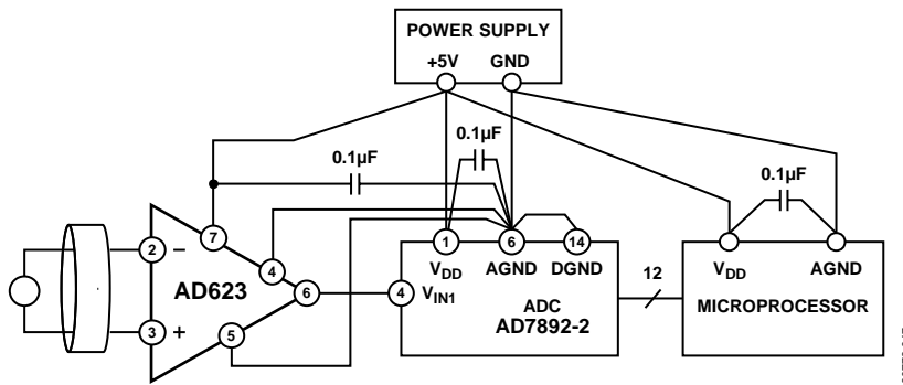
Figure 77. Optimal Ground Practice in a Single-Supply Environment
