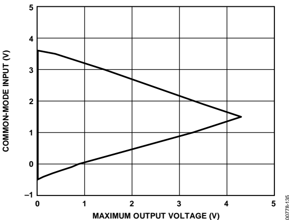
Figure 35. Common-Mode Input vs. Maximum Output Voltage, G = 1 , +V_S = 5 \text{ V} , -V_S = 0 \text{ V} , R_L = 100 \text{ k}\Omega , RM-8 and R-8 Package Options
