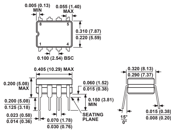
Figure 47. 8-Lead Ceramic DIP - Glass Hermetic Seal [CERDIP] (Q-8) Z-Suffix
