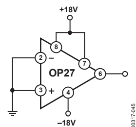
Figure 45. Burn-In Circuit
