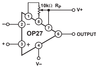
Figure 35. Offset Nulling Circuit
