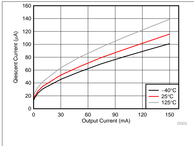
Figure 7. Quiescent Current vs Output Current
