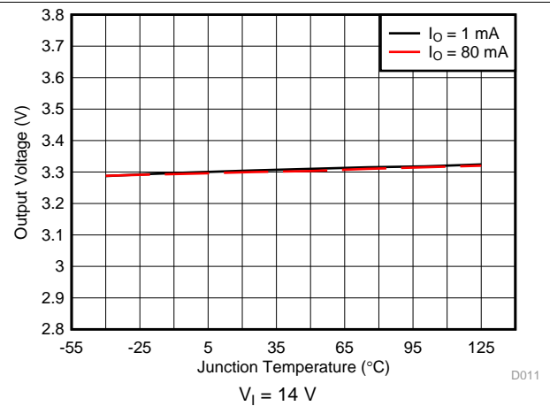
Figure 2. 3.3-V Output Voltage vs Junction Temperature
