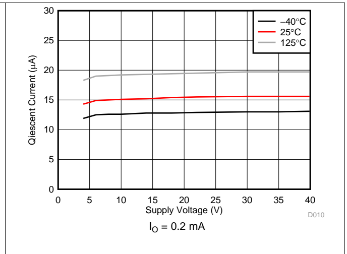
Figure 8. Quiescent Current vs Supply Voltage
