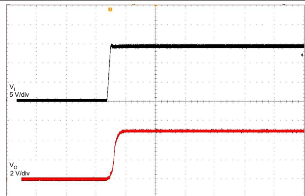
C_O = 2.2 \mu\text{F} , 400 \mu\text{s}/\text{div}
