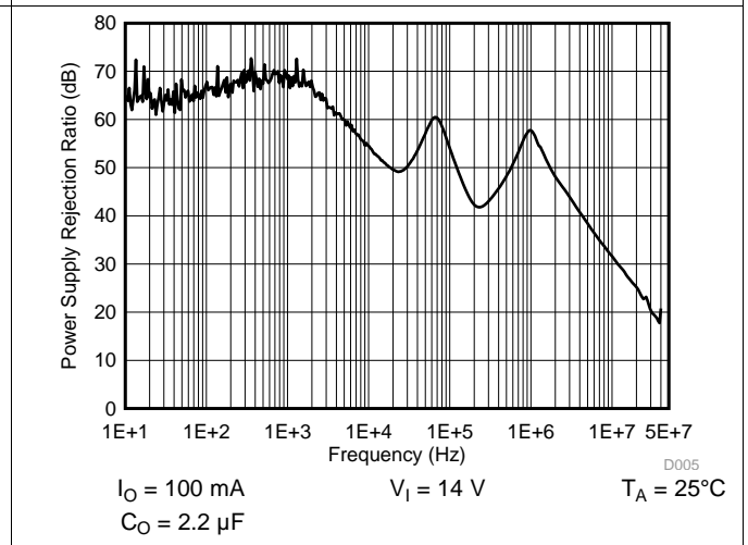
Figure 10. Power Supply Rejection Ratio
