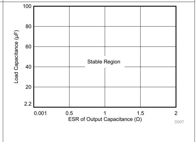
Figure 12. ESR Stability vs Output Capacitance
