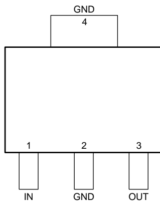
DCY Package 4-Pin SOT-223 Top View
