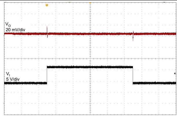
V_I = 9 \text{ to } 16 \text{ V} C_O = 2.2 \mu\text{F} I_O = 10 \text{ mA} 1 ms/div
