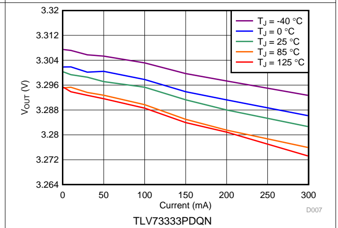
Figure 6. 3.3-V Load Regulation vs I_{OUT} and Temperature
