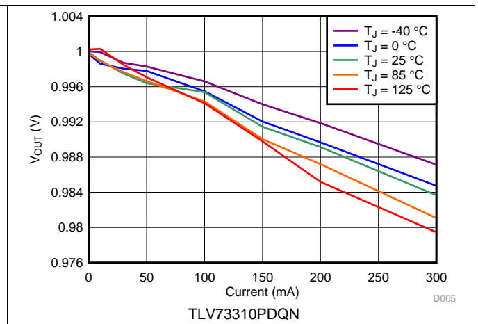
Figure 2. 1.0-V Load Regulation vs I_{OUT} and Temperature
