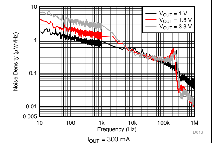
Figure 22. Output Spectral Noise Density
