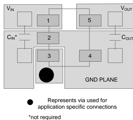
Figure 40. Layout Example for the DBV Package
