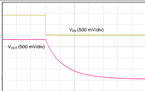
Figure 31. Shutdown Response with Enable
