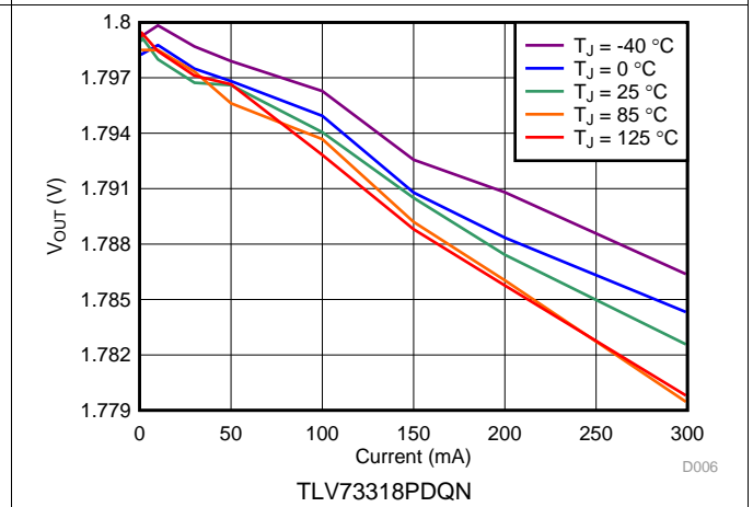
Figure 4. 1.8-V Load Regulation vs I_{OUT} and Temperature
