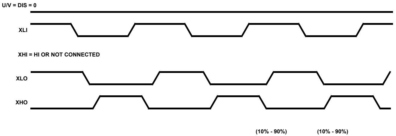
FIGURE 2. BISTATE MODE
