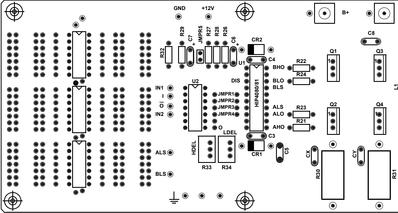
FIGURE 32. HIP4081A EVALUATION BOARD SILKSCREEN
