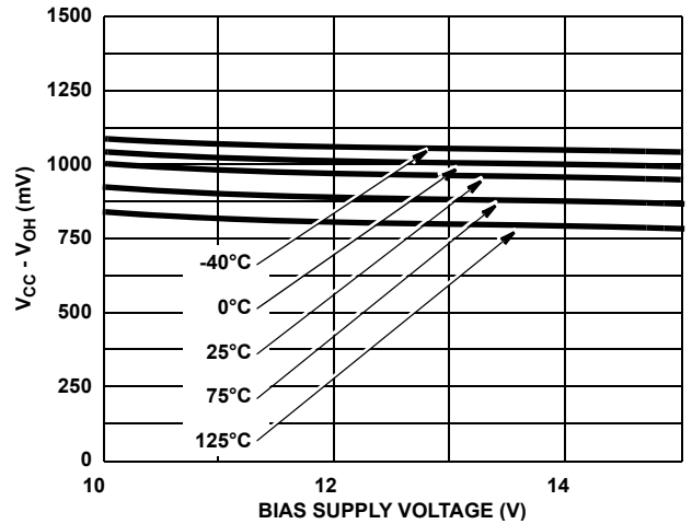
FIGURE 23. HIGH LEVEL OUTPUT VOLTAGE V_{CC} - V_{OH} vs BIAS SUPPLY AND TEMPERATURE AT 100mA
