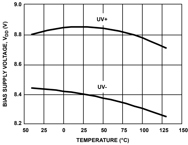
FIGURE 29. UNDERVOLTAGE LOCKOUT vs TEMPERATURE
