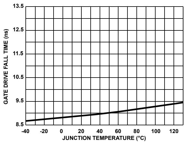
FIGURE 20. GATE DRIVE FALL TIME T_F VS TEMPERATURE
