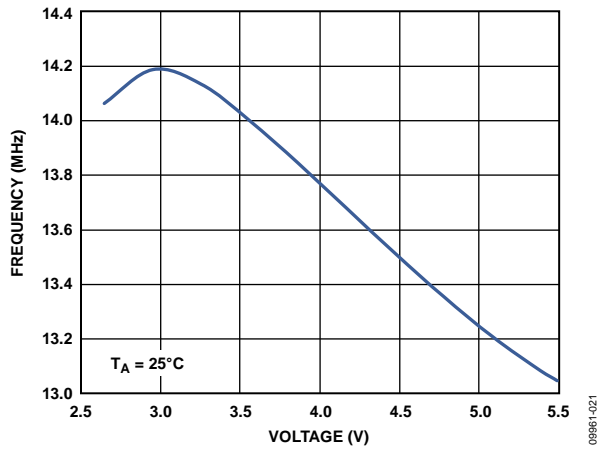
Figure 69. Internal Oscillator Frequency vs. V_{DD} Supply Voltage
