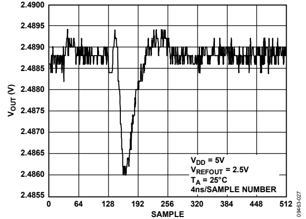
Figure 26. DAC-to-DAC Crosstalk
