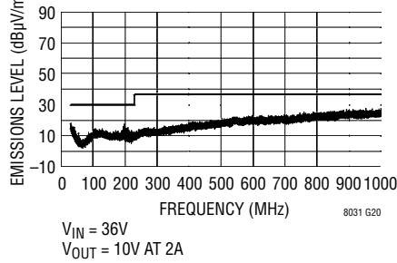
Radiated Emissions
