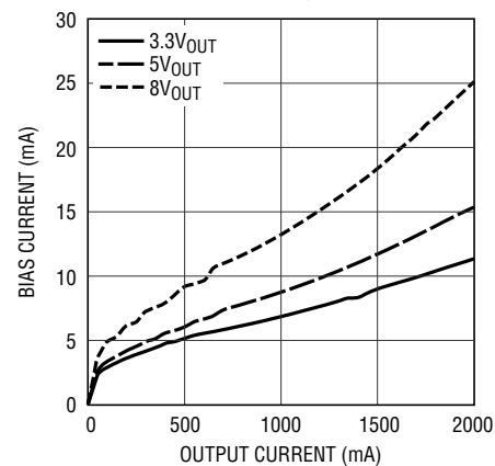
Bias Current vs Output Current
