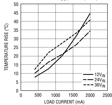
Temperature Rise vs Load Current, V_{OUT} = 8\text{V} (LGA)
