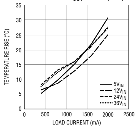
Temperature Rise vs Load Current, V_{OUT} = 2.5\text{V} (LGA)
