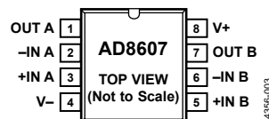
Figure 3. 8-Lead SOIC (R Suffix)
