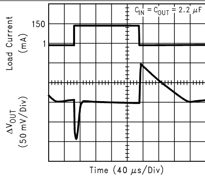
Figure 29. Load Transient Response
