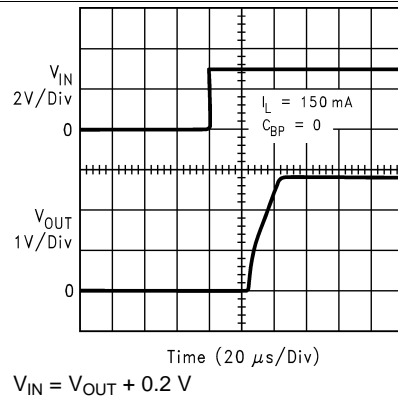
Figure 22. Start-up Time
