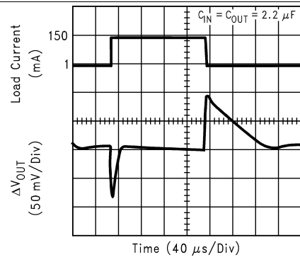
Figure 28. Load Transient Response
