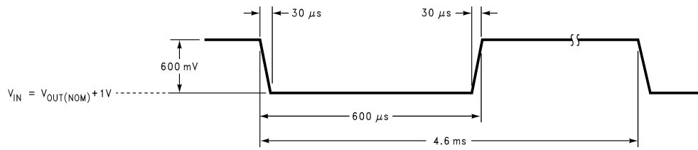
Figure 1. Line Transient Input Test Signal
