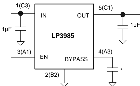
Simplified Schematic
