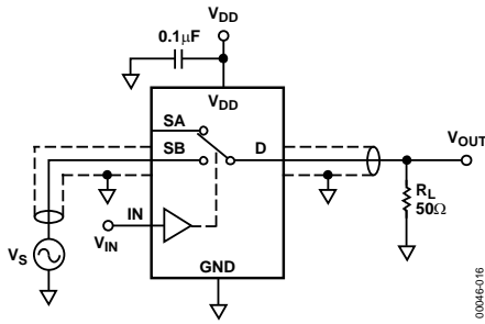
Figure 15. Off Isolation
