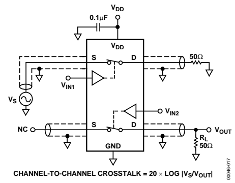
Figure 16. Channel-to-Channel Crosstalk
