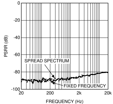
Figure 14. PSRR vs Frequency V_{DD} = 3\text{ V} , R_L = 8\ \Omega V_{RIPPLE} = 200\text{ mV}_{PP} , PV_1 = 4.8\text{ V}
