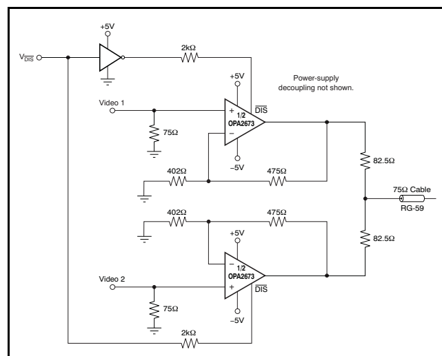
Figure 77. Two-Channel Video Multiplexer
