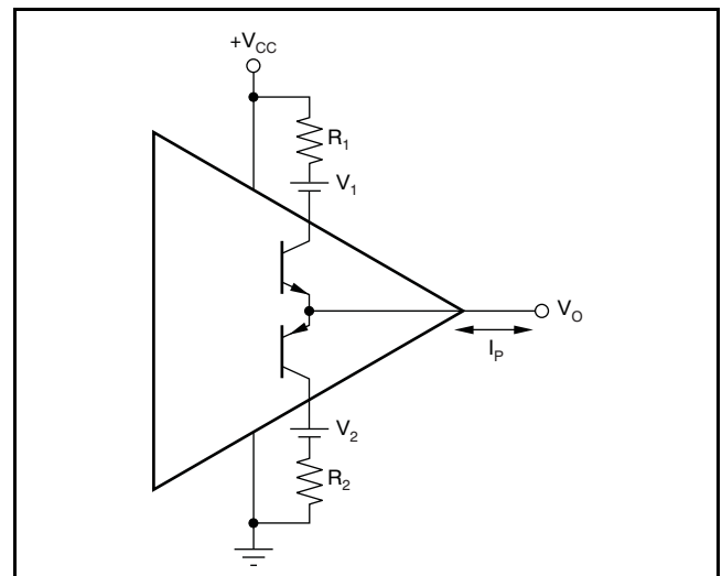
Figure 80. Line Driver Headroom Model
