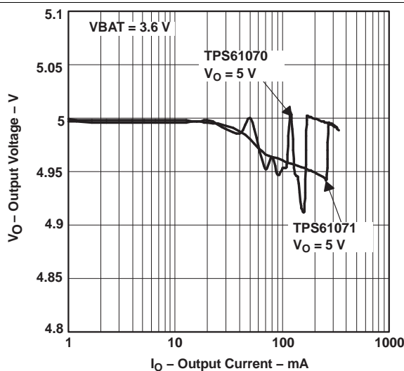
Figure 8. Output Voltage vs Output Current
