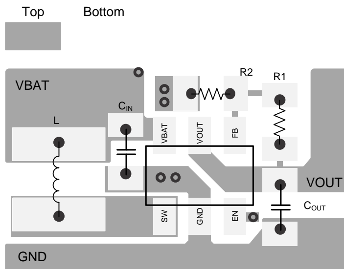
Figure 30. PCB Layout
