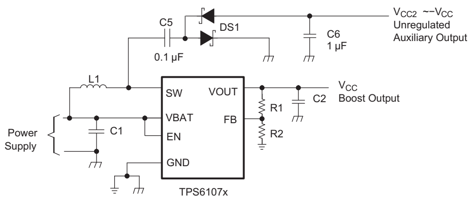
Figure 28. Power Supply Solution With Auxiliary Positive Output Voltage
