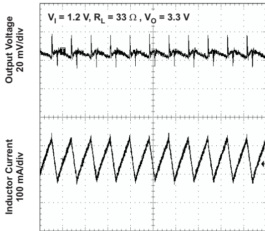
Figure 13. TPS61071 Output Voltage in Continuous Mode
