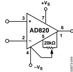
Figure 46. Offset Null
