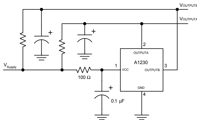
Figure 5: Unregulated Supply
