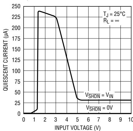
LT1763-5 Quiescent Current
