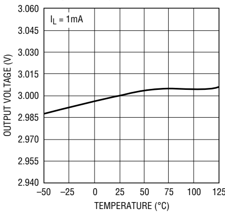
LT1763-3 Output Voltage
