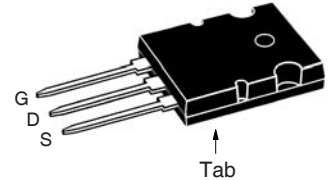
TO-264 (IXFK)
