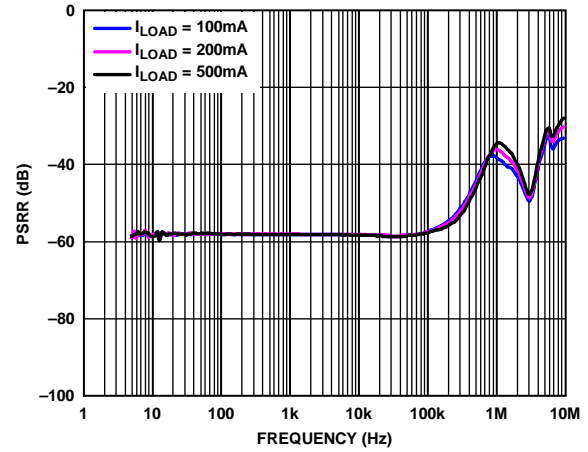
Figure 37. Power Supply Rejection Ratio (PSRR) vs. Frequency, 800 mV Headroom, V_{OUT} = 5 V
