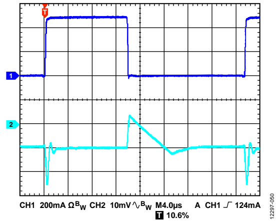
Figure 50. Load Transient Response, I_{LOAD} = 10\text{ mA} to 510\text{ mA} , Adjustable Version, V_{OUT} = 1.2V , V_{IN} = 2.5V , CH1 = I_{LOAD} , CH2 = V_{OUT}
