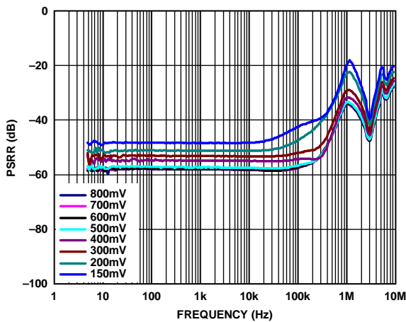
Figure 35. Power Supply Rejection Ratio (PSRR) vs. Frequency, V_{OUT} = 5 V , 500 mA Load Current, Various Headroom Voltages
