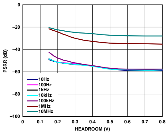
Figure 36. Power Supply Rejection Ratio (PSRR) vs. Headroom, V_{OUT} = 5 V , 500 mA Load Current, Different Frequencies
