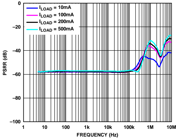
Figure 34. Power Supply Rejection Ratio (PSRR) vs. Frequency, 300 mV Headroom, V_{OUT} = 3 V
