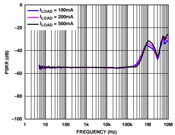
Figure 39. Power Supply Rejection Ratio (PSRR) vs. Frequency, 300 mV Headroom, V_{OUT} = 5 V
