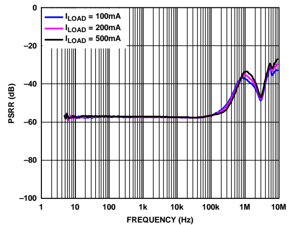
Figure 38. Power Supply Rejection Ratio (PSRR) vs. Frequency, 400 mV Headroom, V_{OUT} = 5 V
