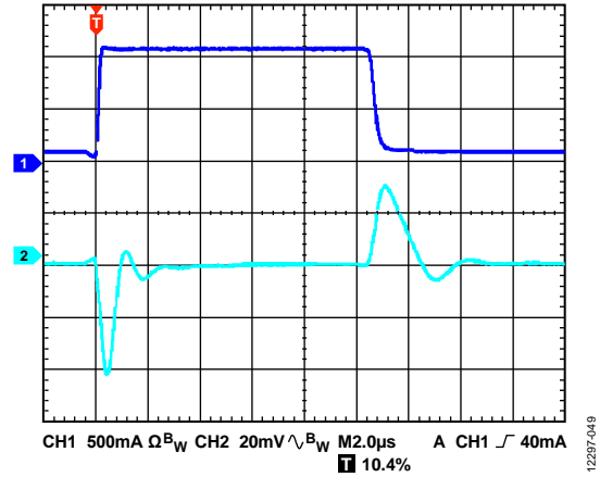
Figure 49. Load Transient Response, I_{LOAD} = 10\text{ mA} to 110\text{ mA} , V_{OUT} = 5V , V_{IN} = 5.5V , CH1 = I_{LOAD} , CH2 = V_{OUT}
