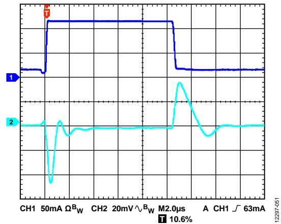
Figure 51. Load Transient Response, I_{LOAD} = 10\text{ mA} to 110\text{ mA} , Adjustable Version, V_{OUT} = 1.2V , V_{IN} = 2.5V , CH1 = I_{LOAD} , CH2 = V_{OUT}
