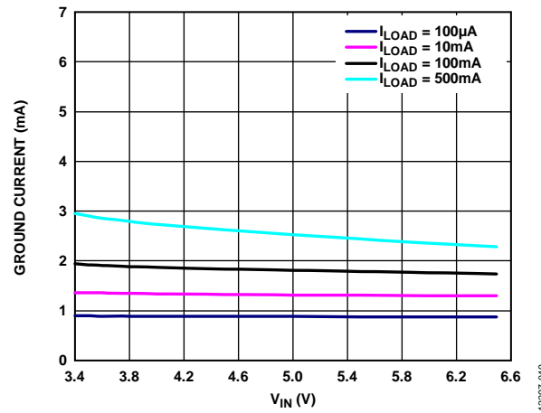
Figure 19. Ground Current vs. Input Voltage ( V_{IN} ), V_{OUT} = 3\text{ V}
