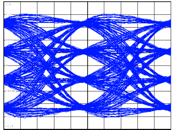
1 Mbps 4-GFSK, 400-kHz Deviation, 300-kHz Loop Bandwidth Figure 4-12. Eye Diagram
