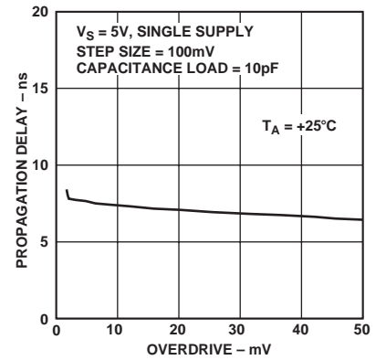
Figure 3. Propagation Delay vs. Overdrive
