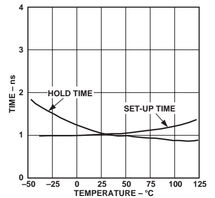
Figure 9. Latch Setup-and-Hold Time vs. Temperature
