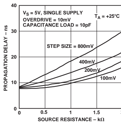
Figure 5. Propagation Delay vs. Source Resistance
