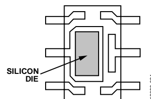
Figure 24. Normal 6-Lead SOT-23 Package
