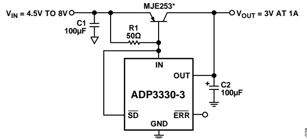
Figure 28. High Output Current Linear Regulator
