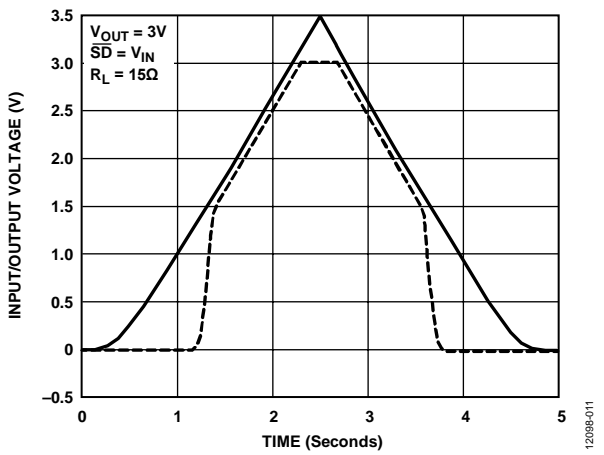
Figure 11. Power-Up/Power-Down
