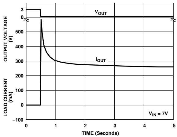
Figure 17. Short-Circuit Current
