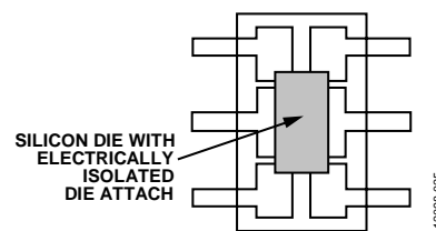
Figure 25. Thermally Enhanced, Chip-on-Lead Package
