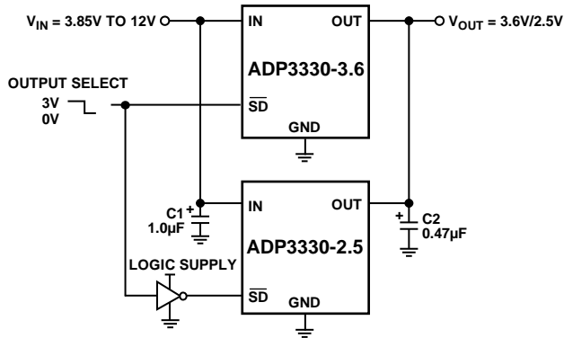
Figure 27. Crossover Switch
