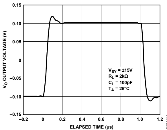
Figure 18. Small Signal Response
