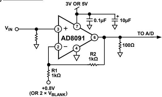
Figure 35. Sync Stripper
