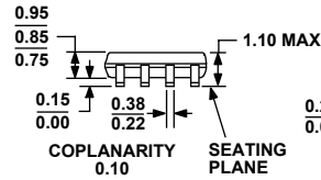
Figure 38. 8-Lead Mini Small Outline Package [MSOP] (RM-8) Dimensions shown in millimeters
