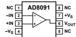
Figure 1. SOIC-8 (R-8)
