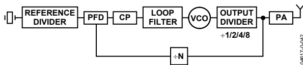
Figure 35. Output Divider Location in PLL
