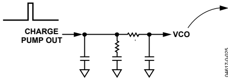
Figure 29. Typical Loop Filter
