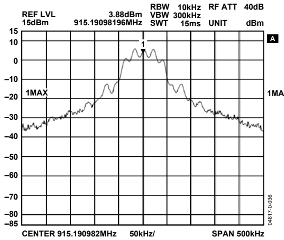
Figure 22. FSK Modulation, Power = 10 dBm, Data Rate = 38.4 kbps, F_{DEVIATION} = \pm 19.2 \text{ kHz}
