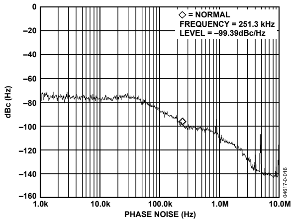
Figure 16. Phase Noise Response— I_{CP} = 2.5 \text{ mA} , I_{VCO} = 1.44 \text{ mA} , R_{FOUT} = 868.95 \text{ MHz} , PF_D = 4.9152 \text{ MHz} , \text{Power} = 12.5 \text{ dBm} , PA \text{ Bias} = \text{Max}
