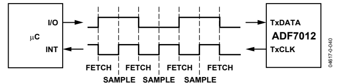
Figure 31. TxCLK/TxDATA Synchronization.
