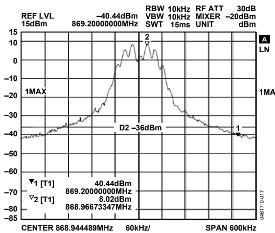
Figure 17. FSK Modulation, \text{Power} = 12.5 \text{ dBm} , \text{Data Rate} = 38.4 \text{ kbps} , F_{\text{DEVIATION}} = \pm 19.2 \text{ kHz}
