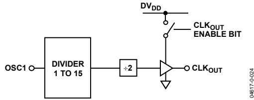
Figure 28. CLKOUT Stage
