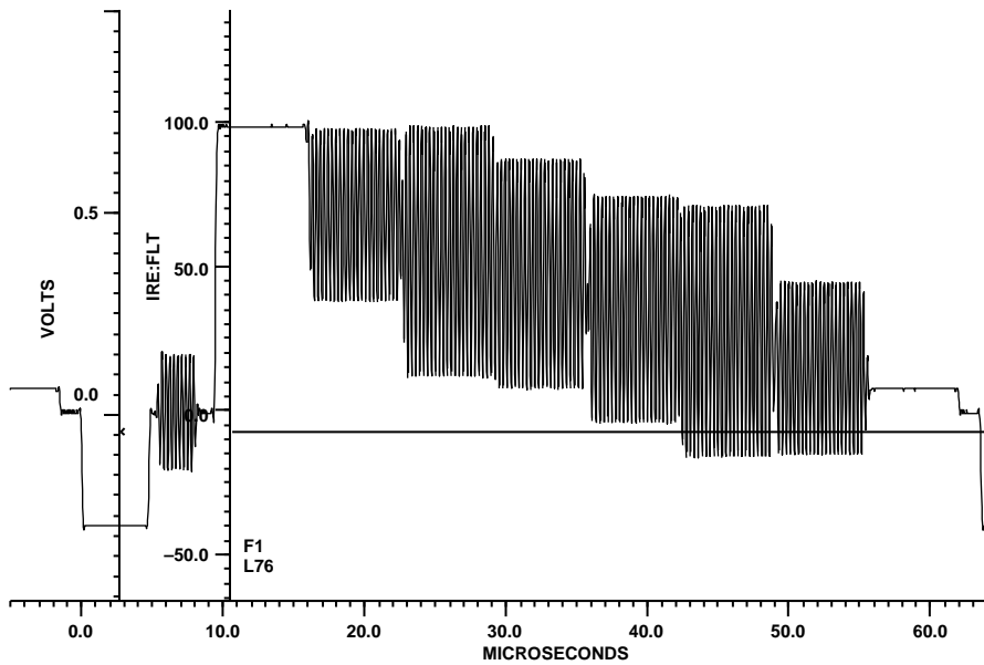
Figure 86. 100/7.5/75/7.5 NTSC Color Bars
