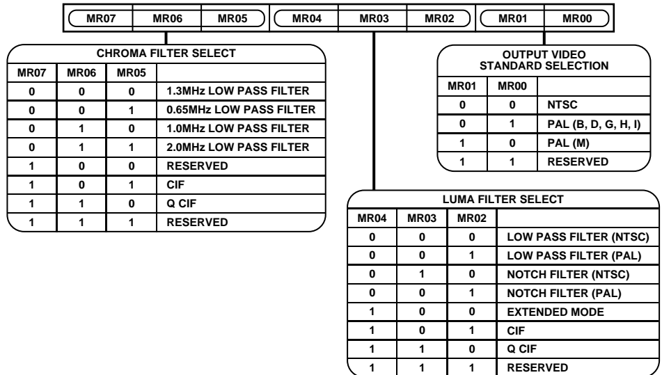
Figure 38. Mode Register 0
