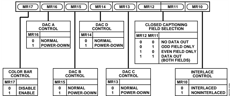
Figure 39. Mode Register 1
