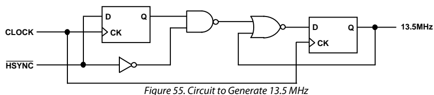
Figure 55. Circuit to Generate 13.5 MHz
