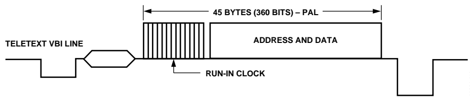
Figure 59. Teletext VBI Line
