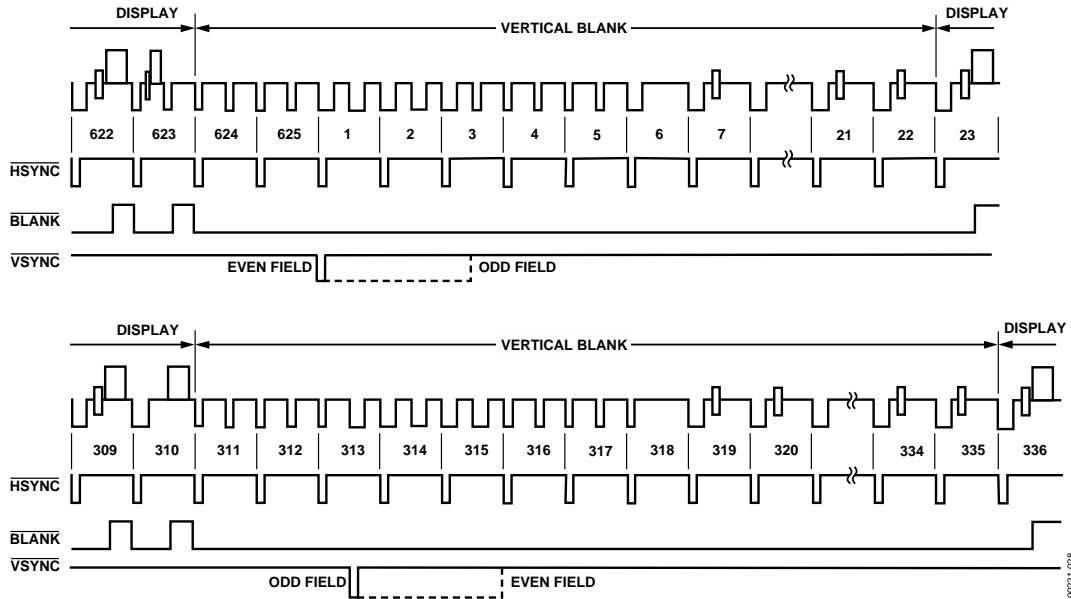
Figure 28. Timing Mode 2 (PAL)
