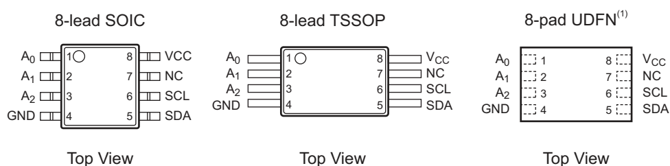
Figure 1-1. Pinouts
