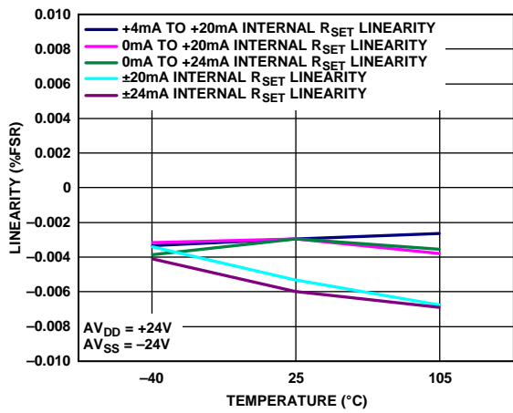
Figure 32. INL vs. Temperature, Internal R_{SET} Sense Resistor
