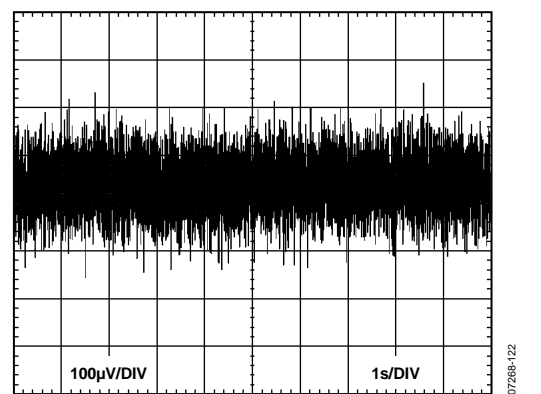
Figure 22. Peak-to-Peak Noise (100 kHz Bandwidth)
