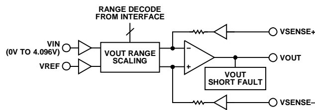
Figure 54. Voltage Output
