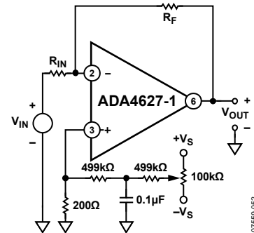
Figure 48. Alternate Offset Null Circuit for Inverting Stage
