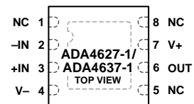
Figure 2. 8-Lead SOIC_N (R-8)
