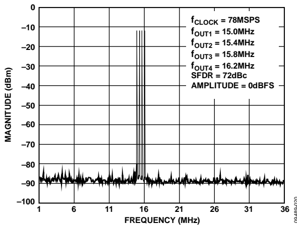
Figure 20. Four-Tone SFDR
