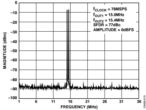
Figure 19. Dual-Tone SFDR
