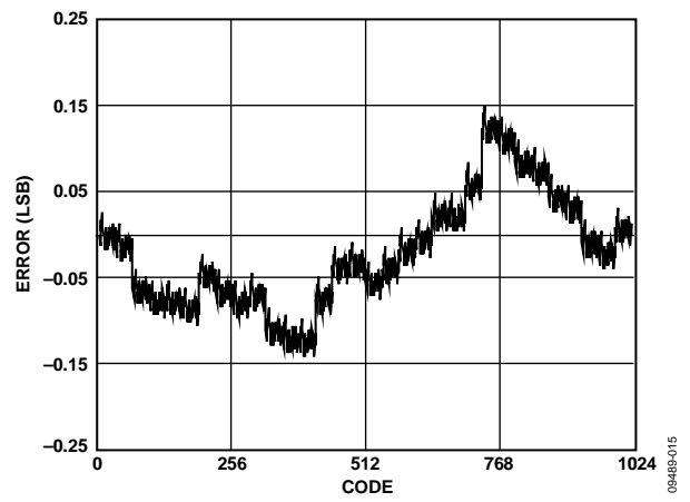
Figure 15. Typical INL
