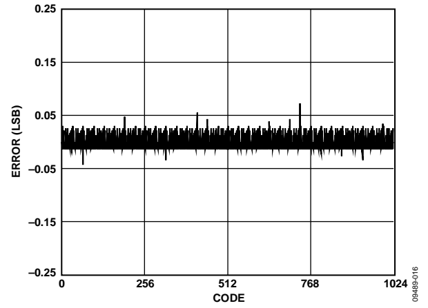
Figure 16. Typical DNL
