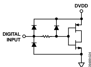
Figure 25. Equivalent Digital Input
