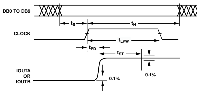
Figure 2. Timing Diagram
