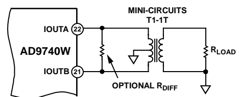
Figure 29. Differential Output Using a Transformer
