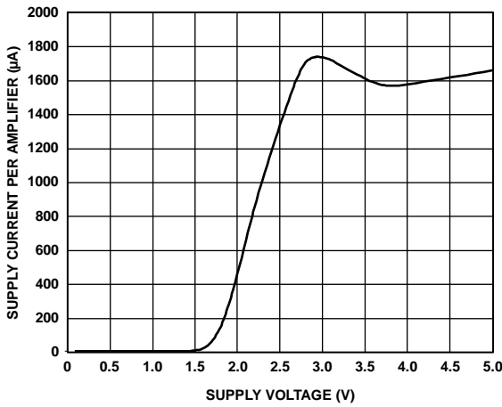
Figure 19. Supply Current per Amplifier vs. Supply Voltage
