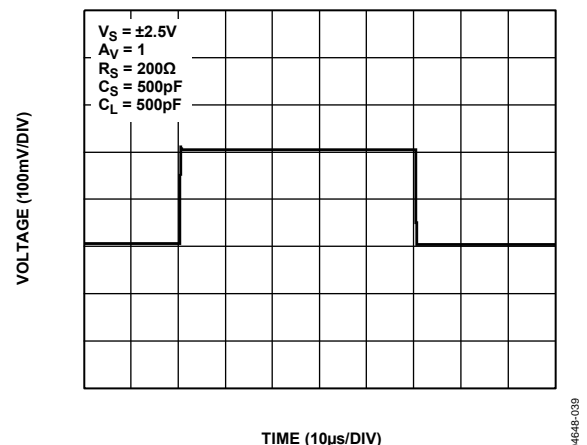
Figure 39. Driving Heavy Capacitive Loads Using the Snubber Network
