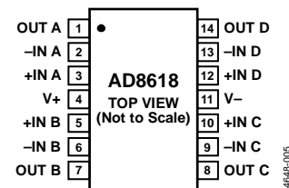
Figure 5. 14-Lead SOIC (R-14)
