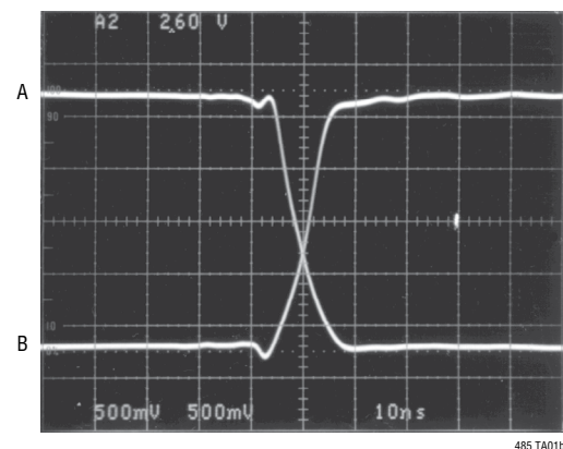
Driver Outputs
