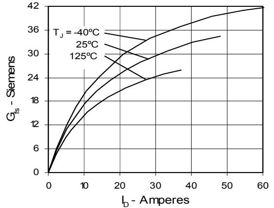
Fig. 8. Transconductance
