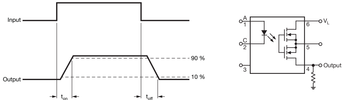
Fig. 2 - Timing Schematic
