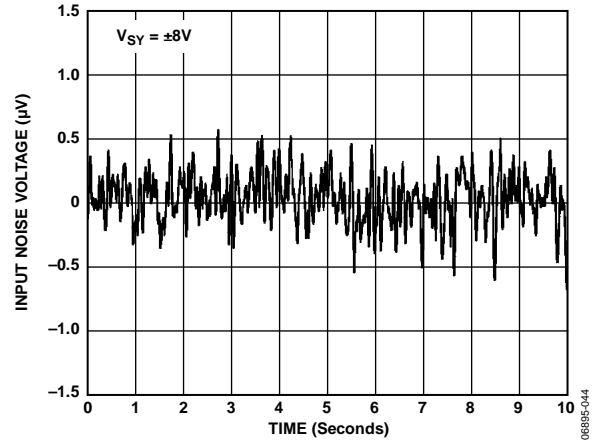
Figure 45. 0.1 Hz to 10 Hz Noise
