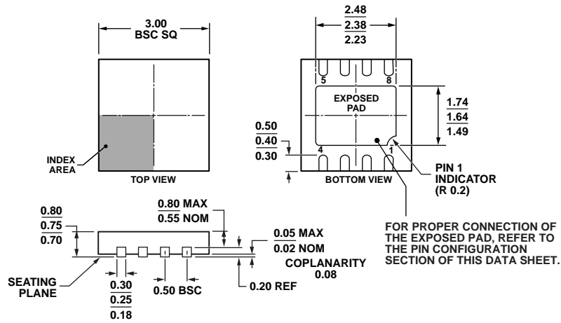
COMPLIANT TO JEDEC STANDARDS MO-229-WEED-4 Figure 58. 8-Lead Lead Frame Chip Scale Package [LFCSP_WD] 3 mm x 3 mm Body, Very Very Thin, Dual Lead (CP-8-5) Dimensions shown in millimeters
