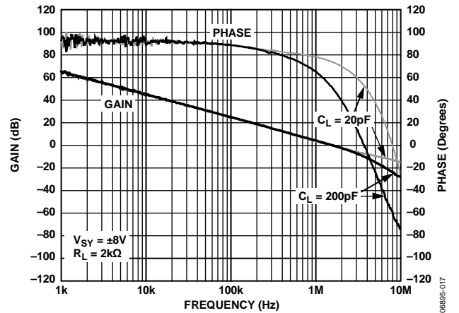
Figure 20. Open-Loop Gain and Phase vs. Frequency
