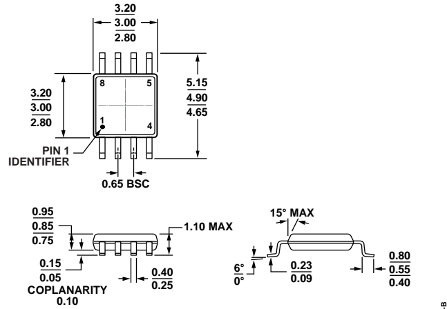
COMPLIANT TO JEDEC STANDARDS MO-187-AA Figure 57. 8-Lead Mini Small Outline Package [MSOP] (RM-8) Dimensions shown in millimeters
