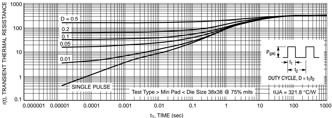
Figure 9. Thermal Response
