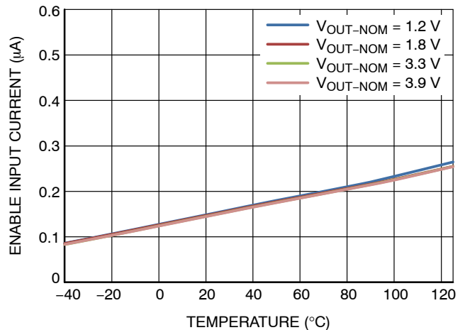
Figure 20. Enable Input Current vs. Temperature
