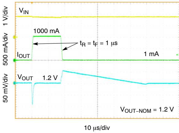
Figure 32. Load Transient Response
