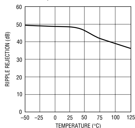
Input Ripple Rejection vs Temperature
