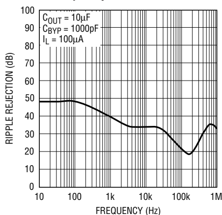
Input Ripple Rejection vs Frequency
