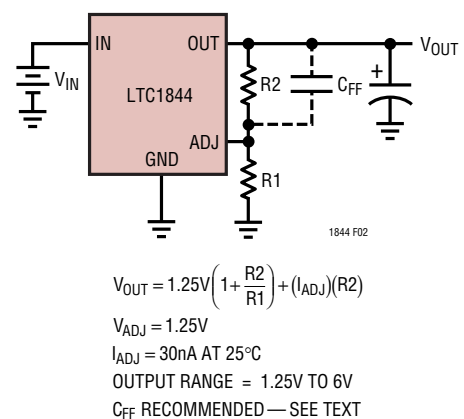
Figure 2. Adjustable Operation
